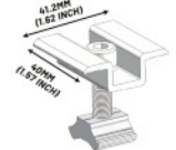
Middle Clamp
