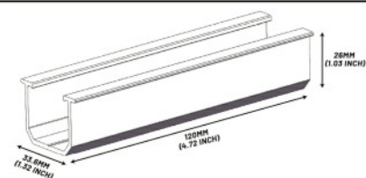
Middle Clamp
